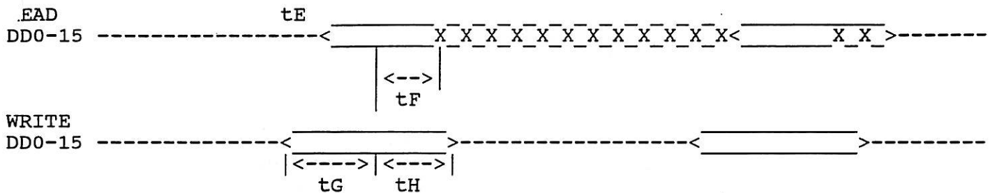
FIGURE 1: Multiword DMA Timing Diagram
