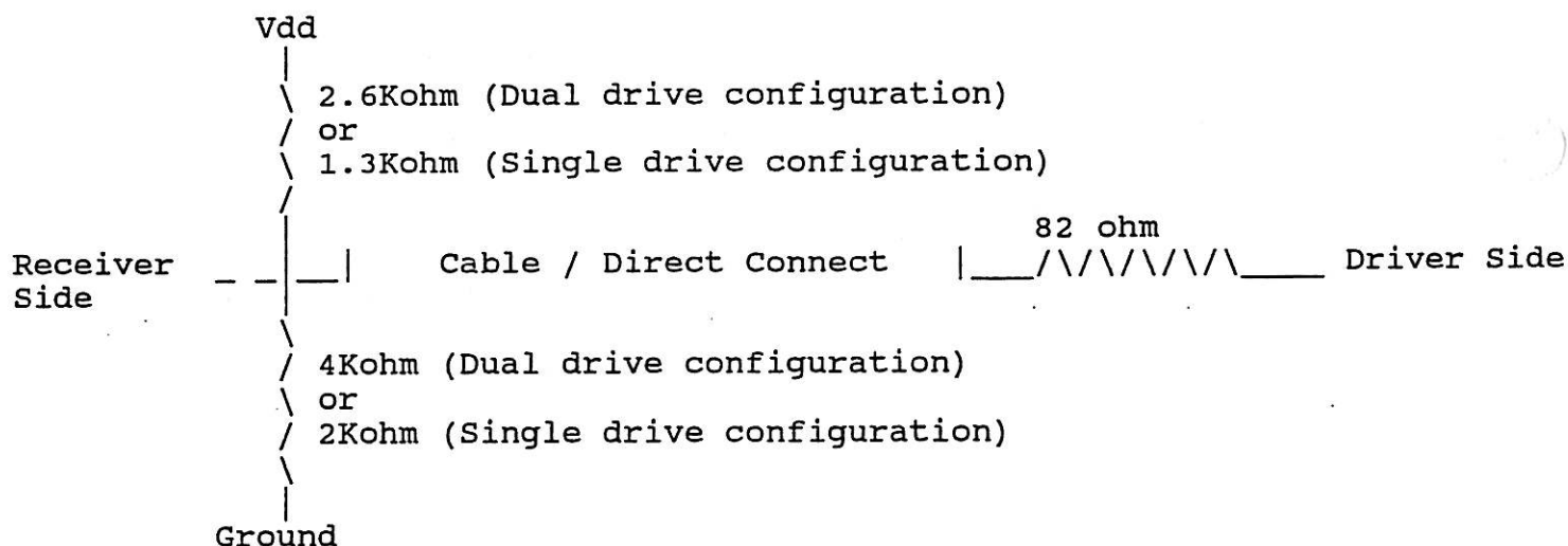
FIGURE 3: Termination Schematic Diagram
